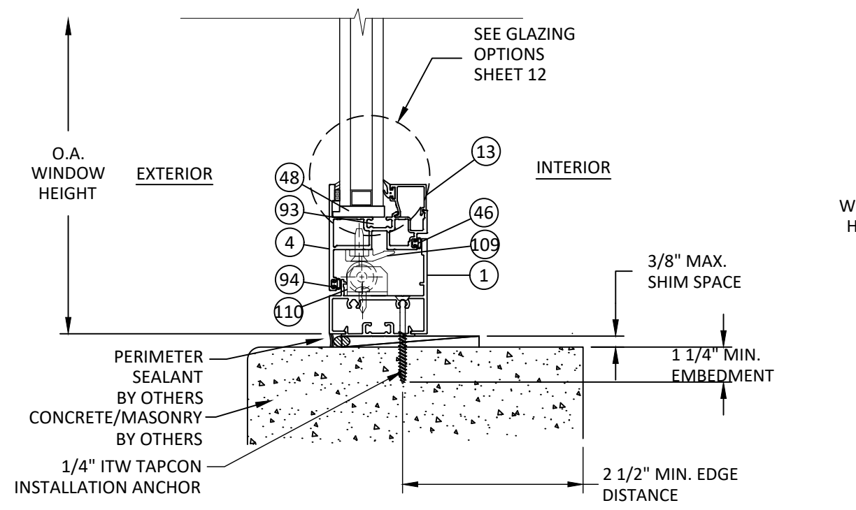
AD 14 VERTICAL SECTION VENT SILL - CONCRETE/MASONRY THROUGH FRAME ANCHOR - TYP. "OUTSWING" - ACCESSIBLE HARDWARE
