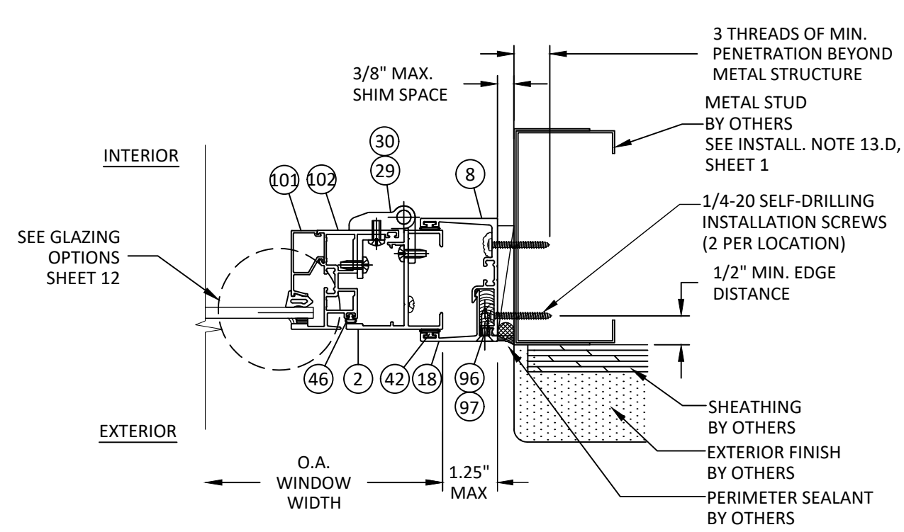
C7 HORIZONTAL SECTION VENT JAMB - METAL STUD FRAME INT. SET RECEPTOR - TYP. "INSWING"
