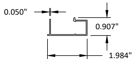
67 STRAP ANCHOR COVER
