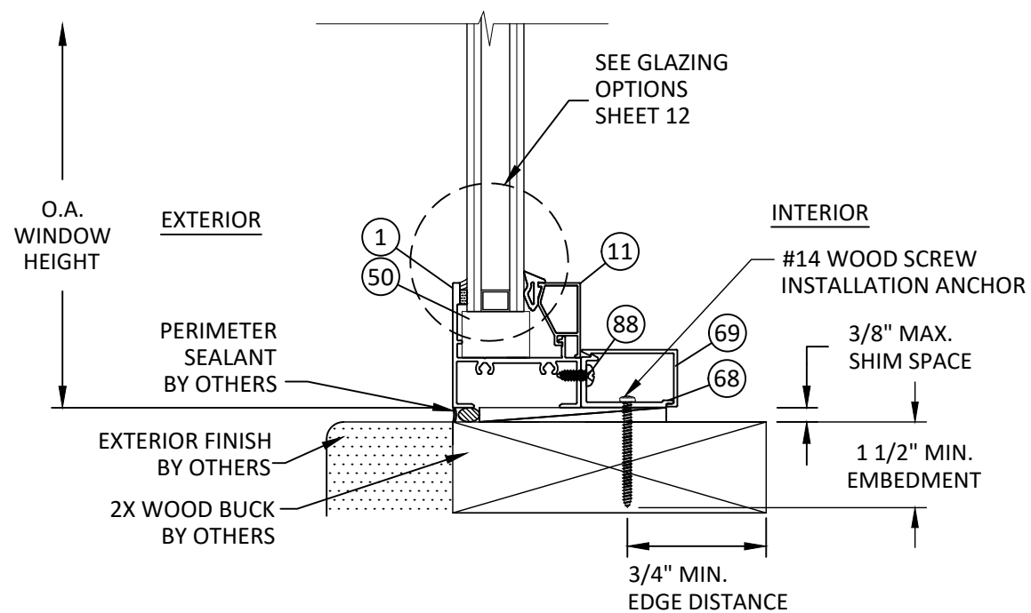
U 11 VERTICAL SECTION FIXED SILL - 2X WOOD BUCK TRIM CLIP ANCHOR - TYP. "FIXED"
