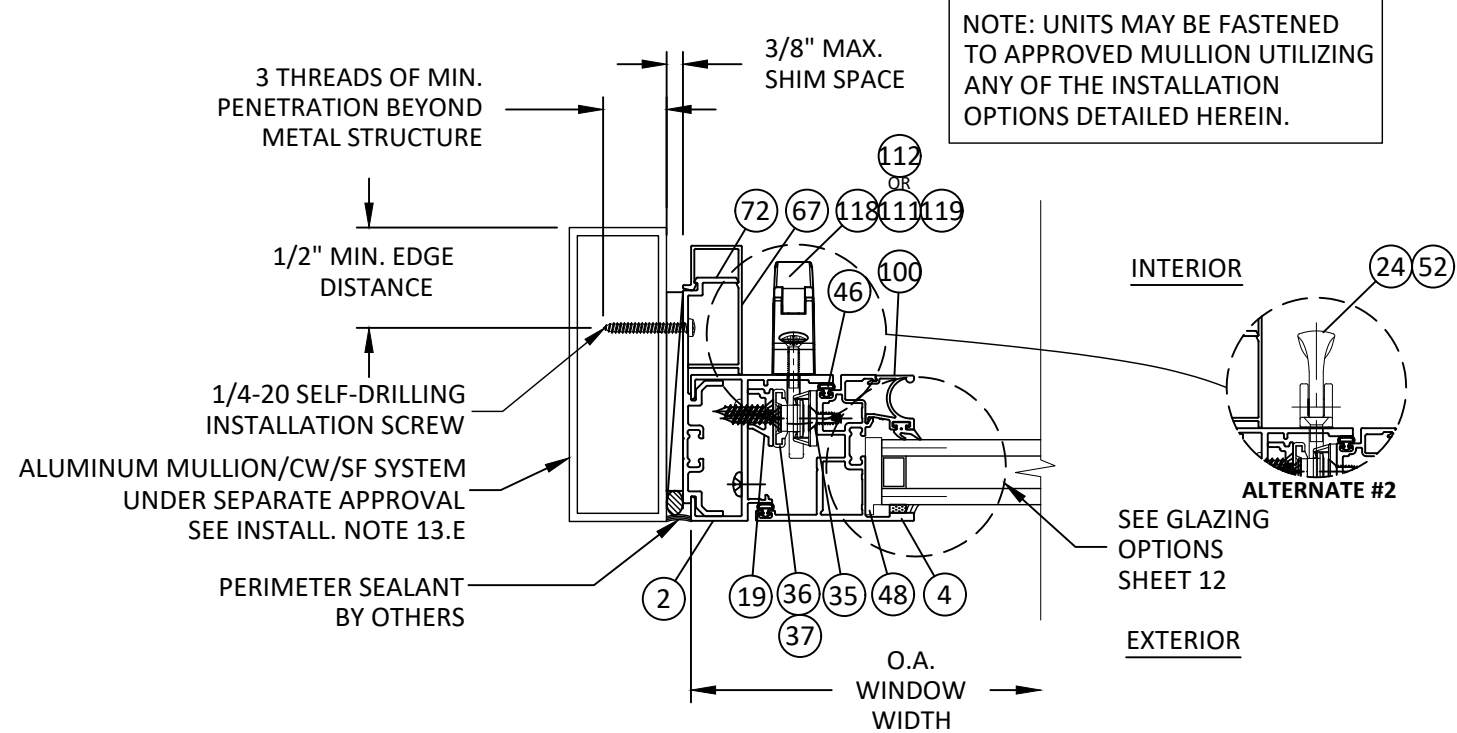
L 9 HORIZONTAL SECTION VENT JAMB - MULL TUBE FRAME STRAP ANCHOR - TYP. "OUTSWING" ALTERNATE #1
