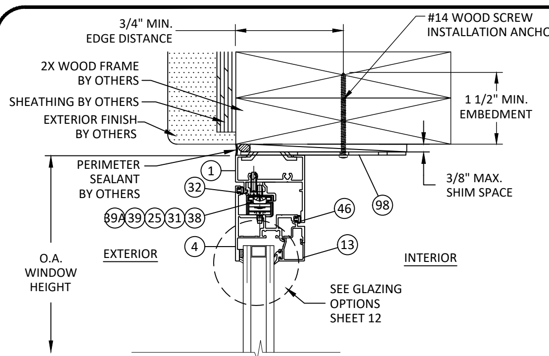
W 12 VERTICAL SECTION VENT HEAD - 2X WOOD FRAME TWIST ANCHOR - TYP. "OUTSWING"
