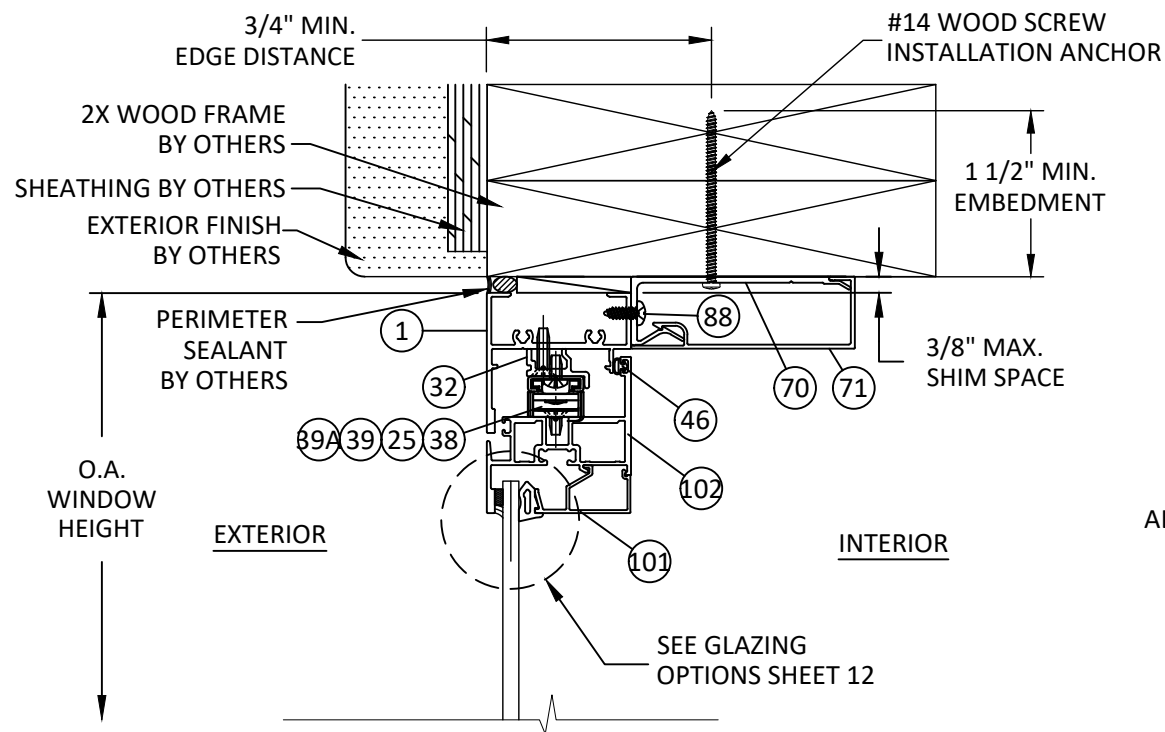
S 11 VERTICAL SECTION VENT HEAD - 2X WOOD FRAME TRIM CLIP ANCHOR - TYP. "INSWING"
