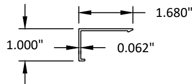
69 1" X 1 11/16" COVER
