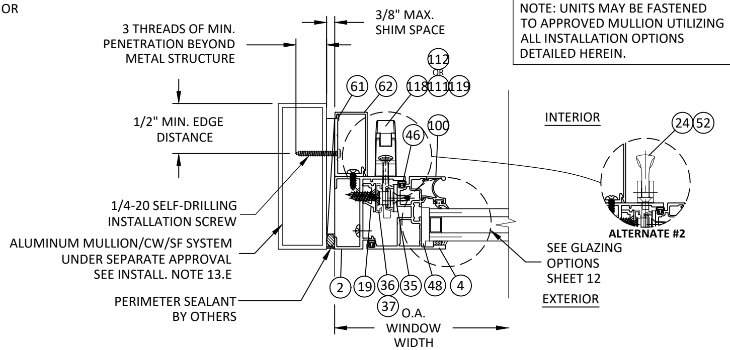
T 11 HORIZONTAL SECTION VENT JAMB - MULL TUBE FRAME TRIM CLIP ANCHOR - TYP. "OUTSWING" ALTERNATE #1
