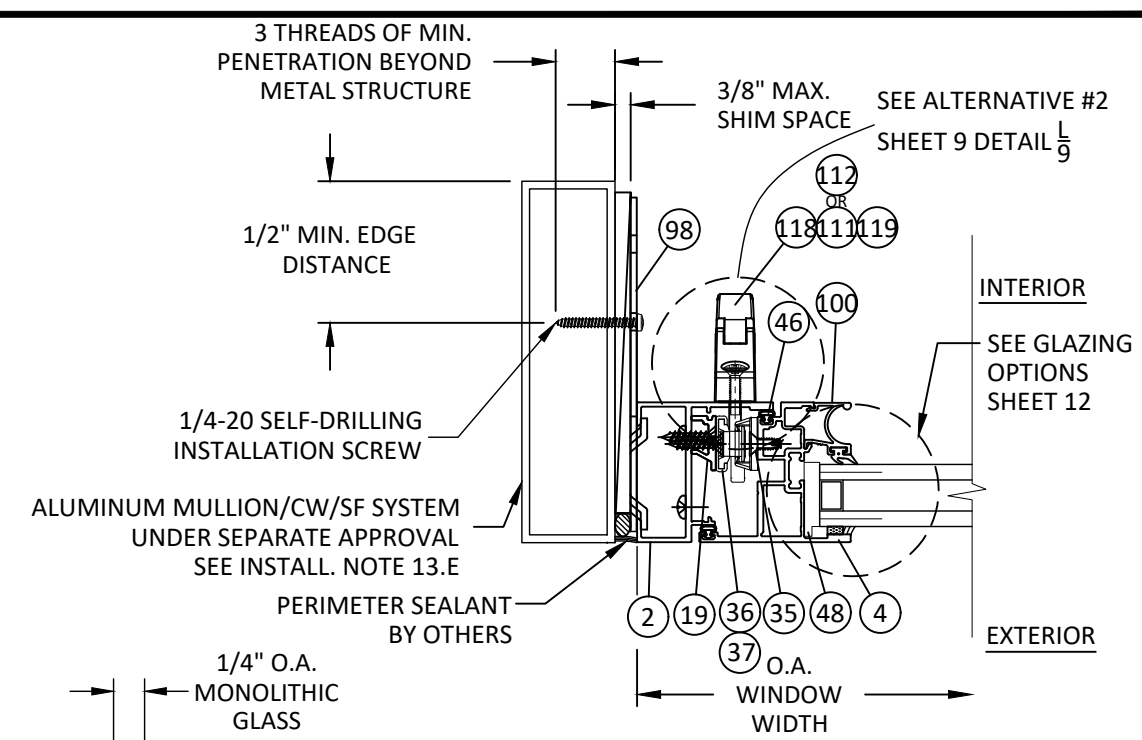
X 12 HORIZONTAL SECTION VENT JAMB - MULL TUBE FRAME TWIST ANCHOR - TYP. "OUTSWING" ALTERNATE #1
