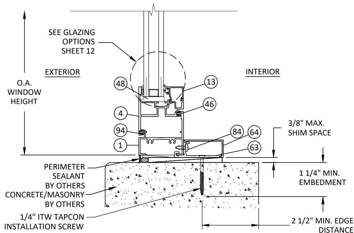
F 8 VERTICAL SECTION VENT SILL - CONCRETE/MASONRY CLIP ANCHOR - TYP. "OUTSWING"
