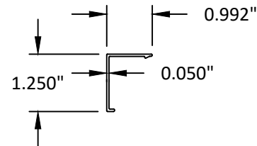
66 1 1/4" X 1" COVER
