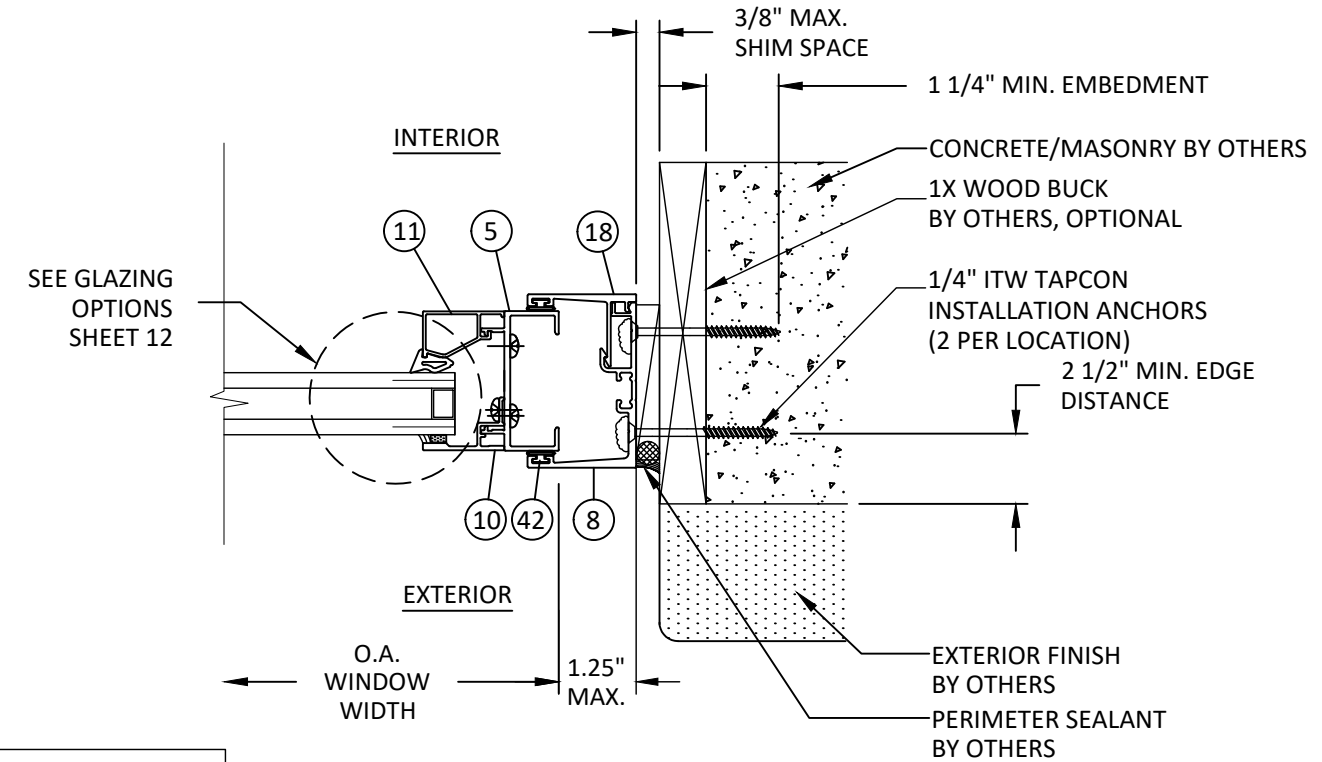
D7 HORIZONTAL SECTION FIXED JAMB - 1X/CONCRETE/MASONRY EXT. SET RECEPTOR - TYP. "FIXED"
