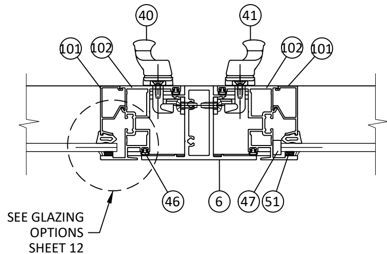
AQ 18 HORIZONTAL SECTION MEETING STILE "INSWING"
