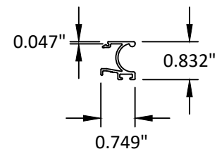
100 VENT GLASS STOP WITH PULL
