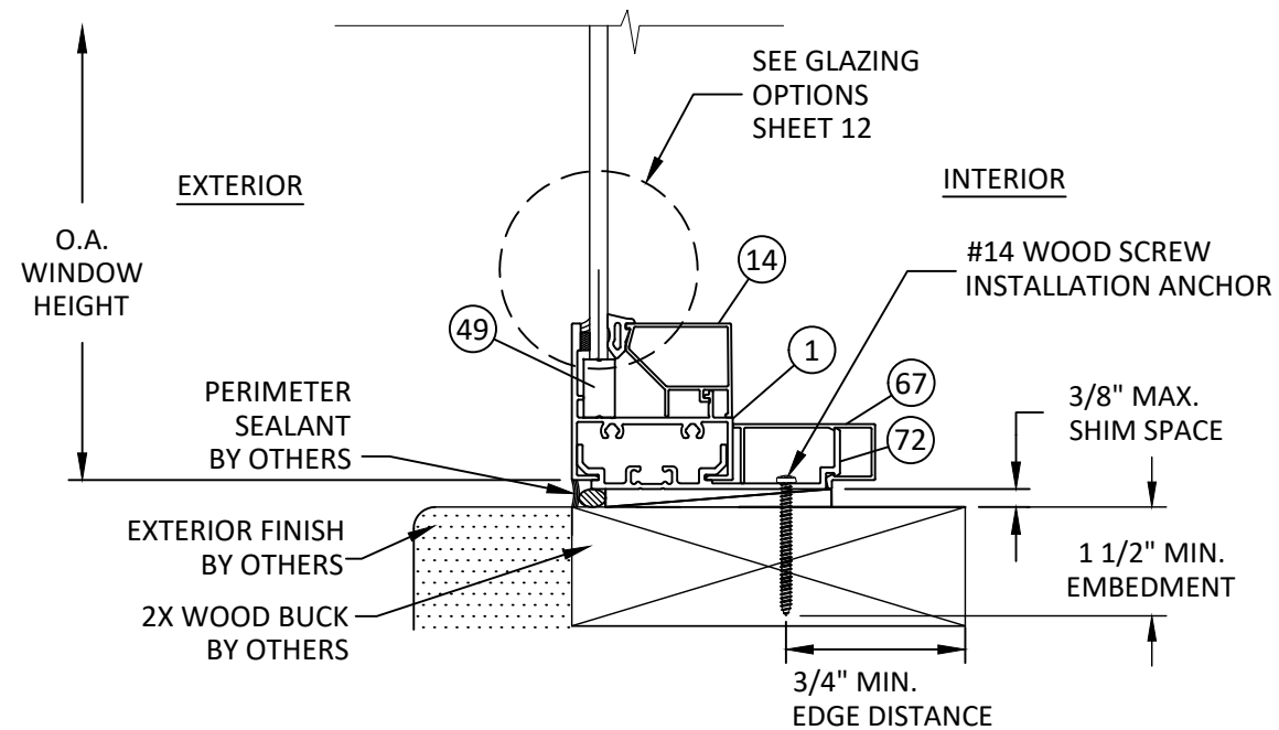
M 9 VERTICAL SECTION FIXED SILL - 2X WOOD BUCK STRAP ANCHOR - TYP. "FIXED"
