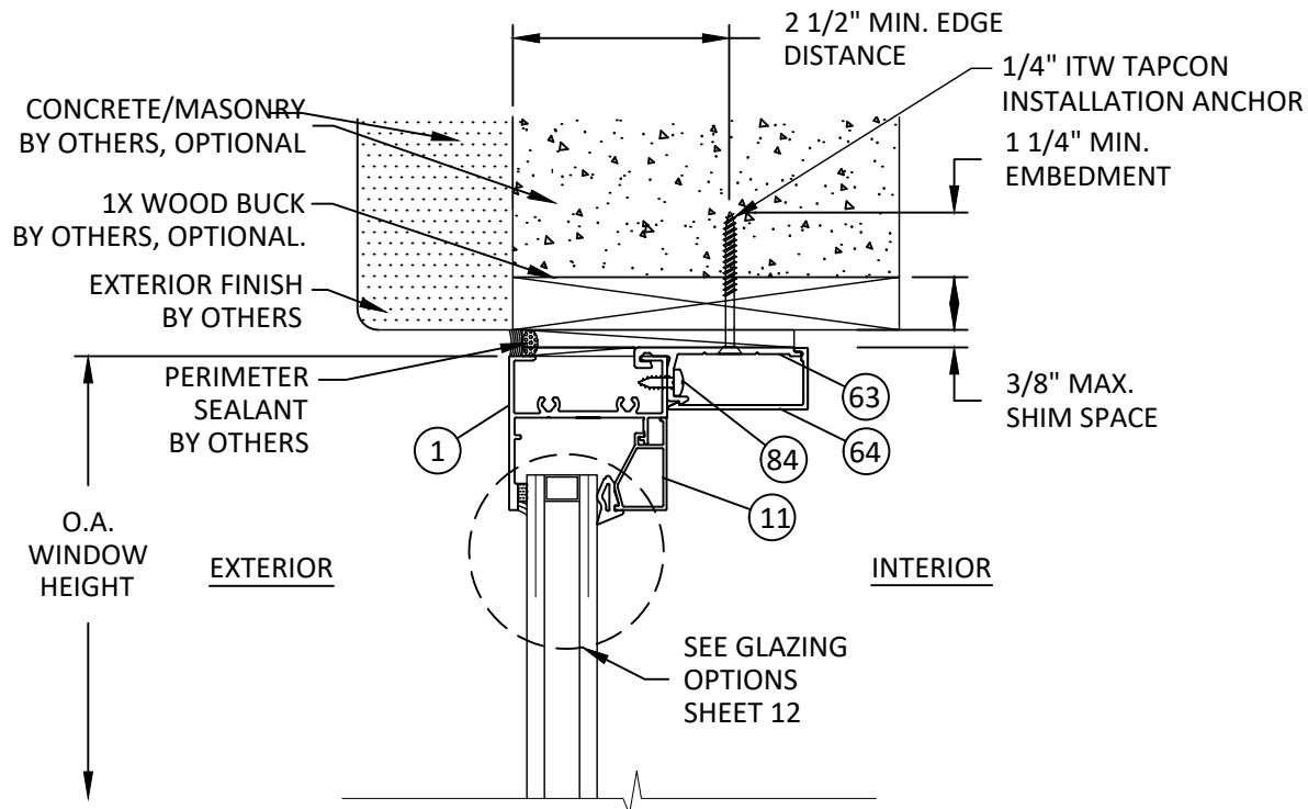
H 8 VERTICAL SECTION FIXED HEAD - 1X/CONCRETE/MASONRY CLIP ANCHOR - TYP. "FIXED"
