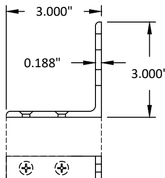
73 MULLION CLIP
