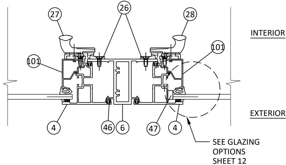
AJ HORIZONTAL SECTION 16 MEETING STILE "OUTSWING"
