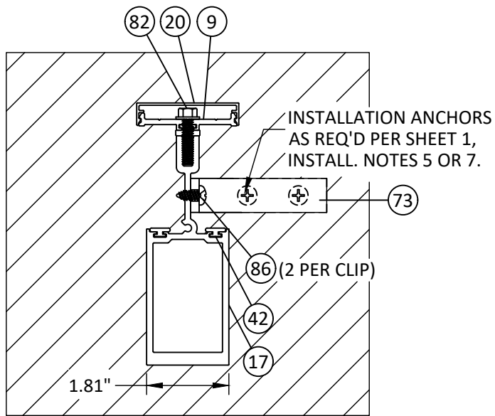
AU 18 HORIZONTAL SECTION STACK MULLION - TYP. JAMB INSTALLATION INSTALL TO WOOD/METAL FRAME
