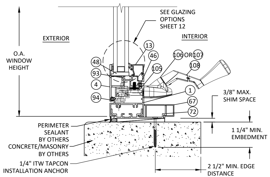
AC 13 VERTICAL SECTION VENT SILL - CONCRETE/MASONRY STRAP ANCHOR - TYP. "OUTSWING" - ACCESSIBLE HARDWARE
