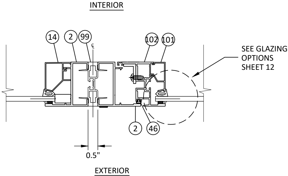
AP 17 HORIZONTAL SECTION "I" MULLION - TYP. FIXED TO CASEMENT "INSWING"
