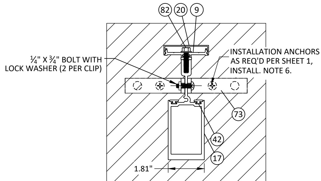
AV 18 HORIZONTAL SECTION STACK MULLION - TYP. INTERMEDIATE INSTALLATION INSTALL TO CONCRETE/MASONRY
