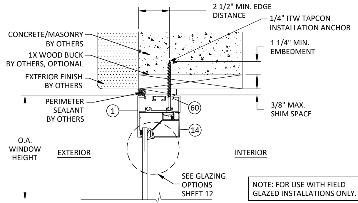
P 10 VERTICAL SECTION FIXED HEAD - 1X/CONCRETE/MASONRY THROUGH FRAME - TYP. "FIXED"
