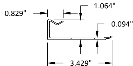
70 1 1/8" X 3 1/2" CLIP
