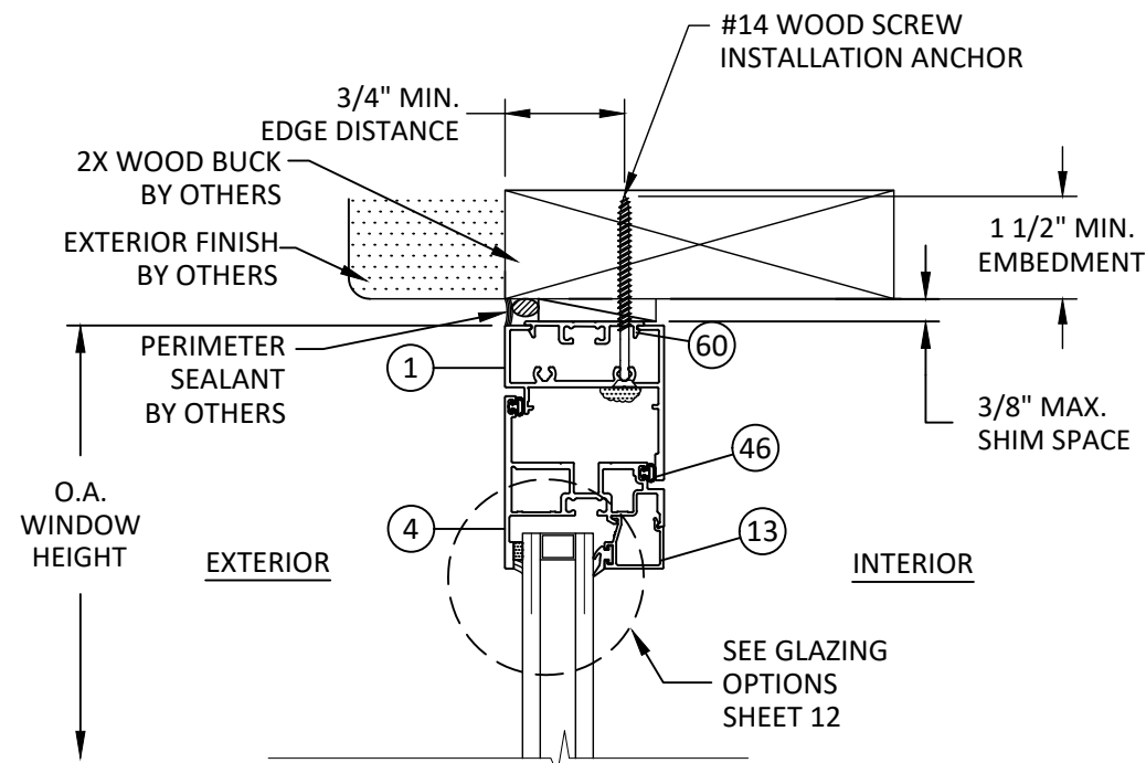
O 10 VERTICAL SECTION VENT HEAD - 2X WOOD BUCK THROUGH FRAME- TYP. "OUTSWING"
