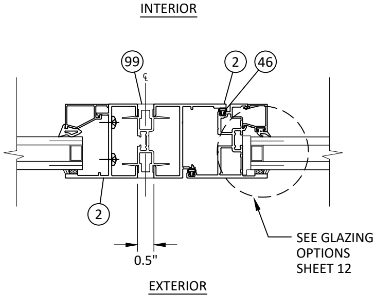
AO 17 HORIZONTAL SECTION "I" MULLION - TYP. FIXED TO CASEMENT "OUTSWING"
