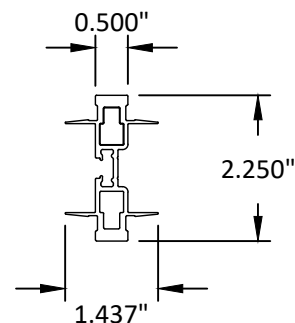
99 I MULLION
