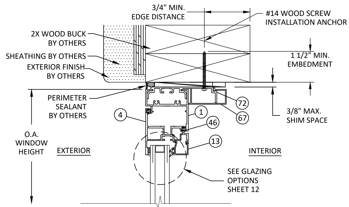
AA 13 VERTICAL SECTION VENT HEAD - 2X WOOD FRAME STRAP ANCHOR - TYP. "OUTSWING" - ACCESSIBLE HARDWARE
