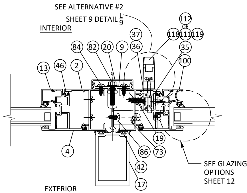
AM HORIZONTAL SECTION 16 STACK MULLION - TYP. CASEMENT TO CASEMENT "OUTSWING" ALTERNATE #1
