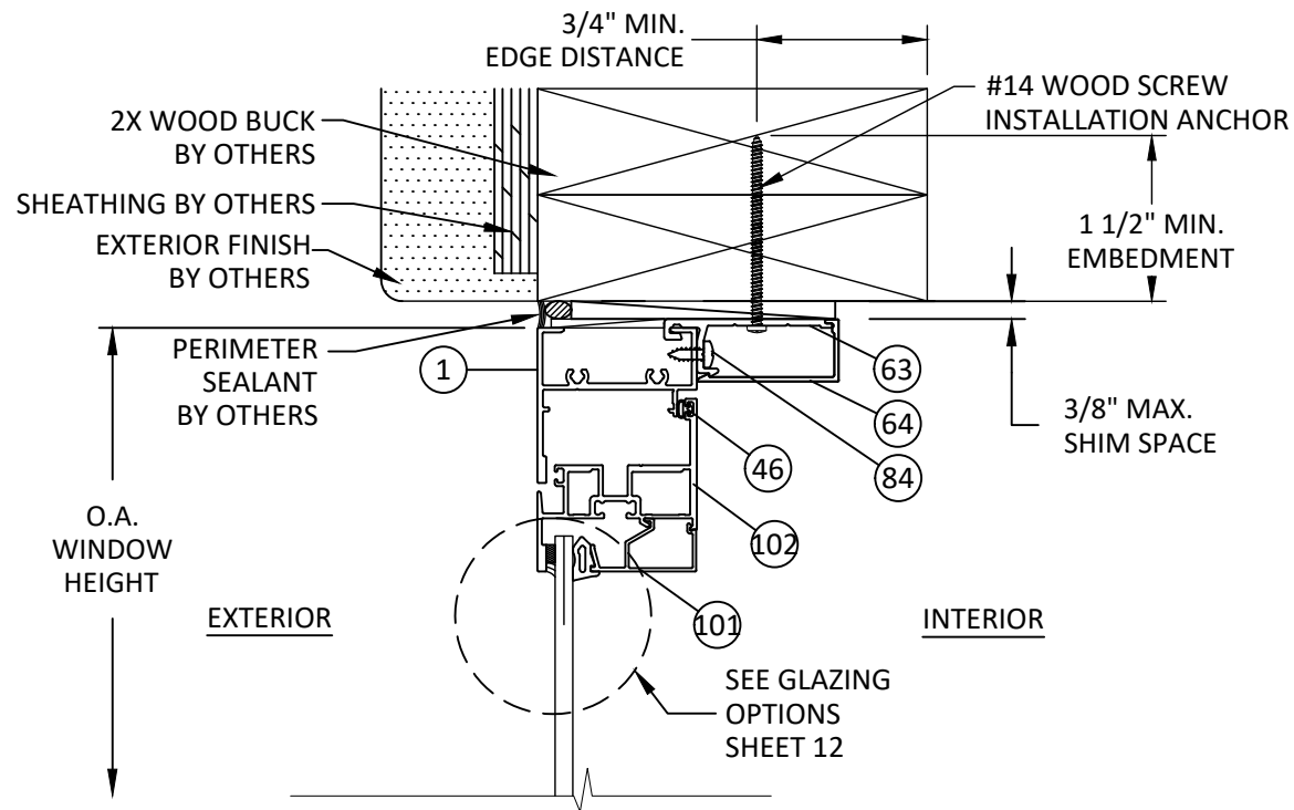
G 8 VERTICAL SECTION VENT HEAD - 2X WOOD FRAME CLIP ANCHOR - TYP. "INSWING"
