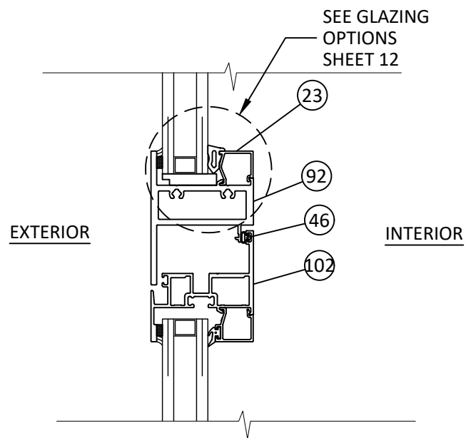
AR 18 VERTICAL SECTION INTEGRAL MULLION-TYP. FIXED OVER CASEMENT "INSWING"
