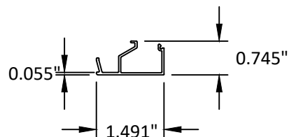
101 VENT GLASS STOP
