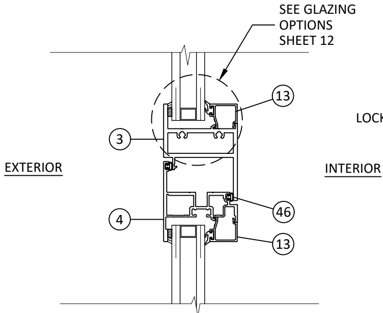
AI VERTICAL SECTION 16 INTEGRAL MULLION-TYP. FIXED OVER CASEMENT "OUTSWING"
