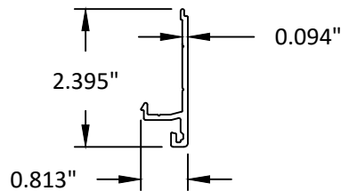
63 ANCHOR CLIP
