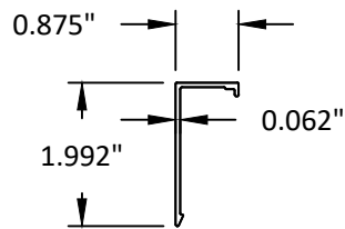
64 ANCHOR CLIP COVER
