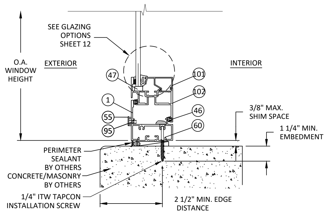
N 10 VERTICAL SECTION VENT SILL - CONCRETE/MASONRY THROUGH FRAME - TYP. "INSWING"
