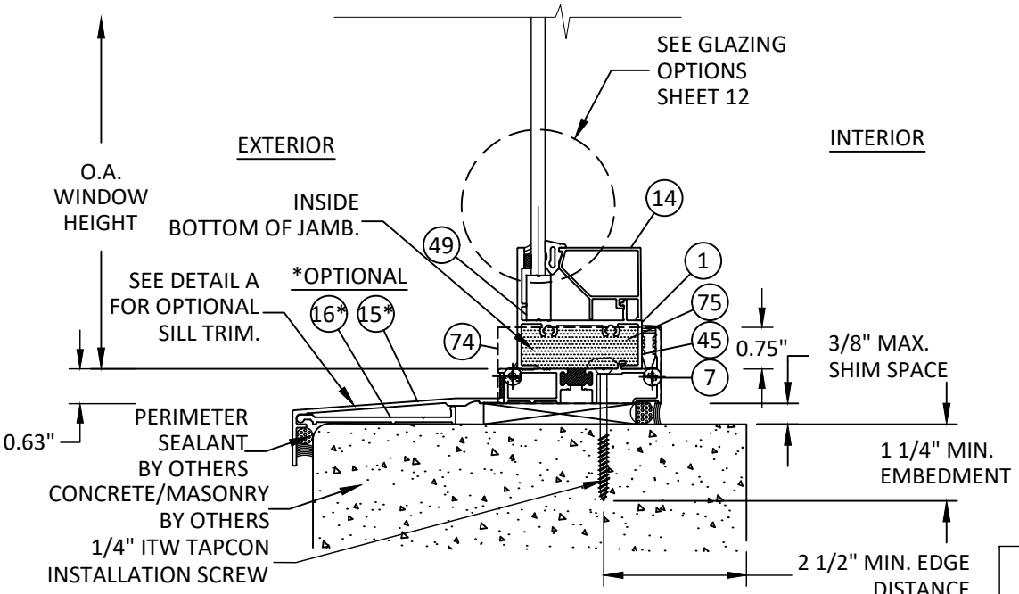
A7 VERTICAL SECTION FIXED SILL - CONCRETE/MASONRY SILL FLASHING - TYP. "FIXED"
