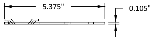
98 TWIST ANCHOR
