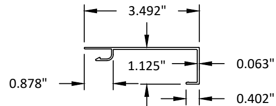
71 1 1/8" X 3 1/2" COVER
