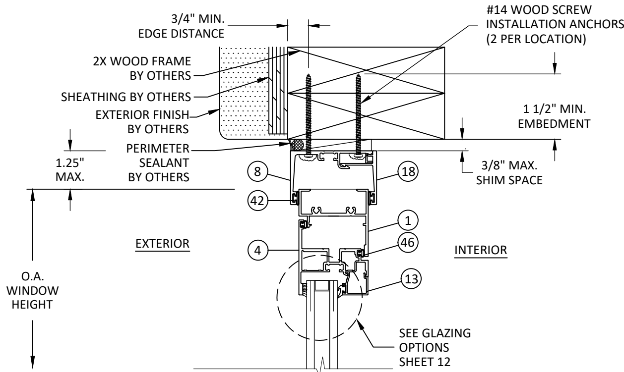
B7 VERTICAL SECTION VENT HEAD - 2X WOOD FRAME INT. SET RECEPTOR - TYP. "OUTSWING"
