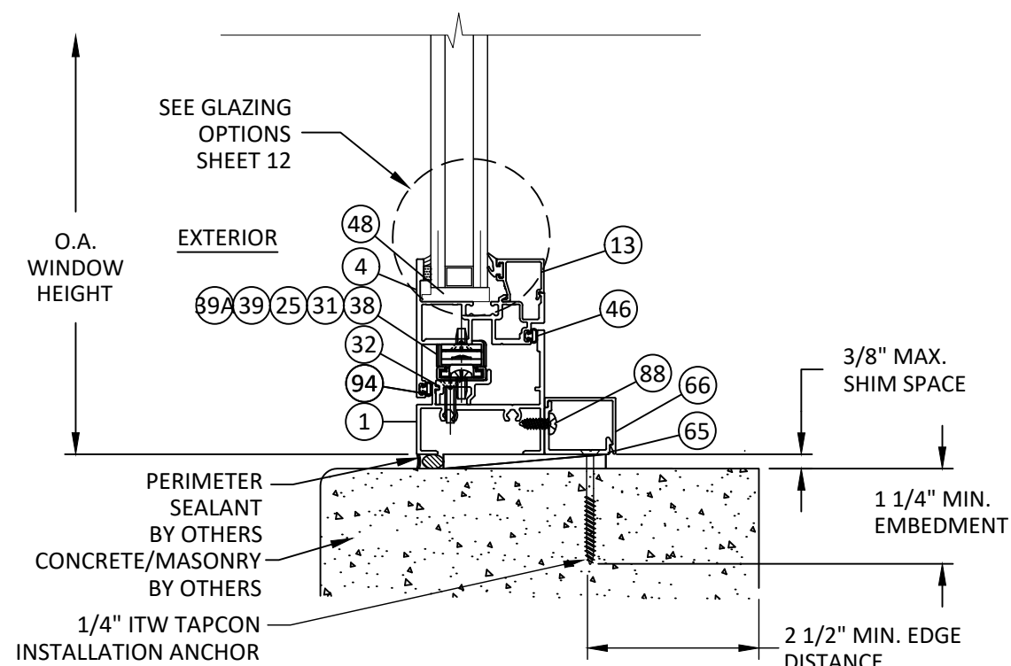
R 11 VERTICAL SECTION VENT SILL - CONCRETE/MASONRY TRIM CLIP ANCHOR - TYP. "OUTSWING"
