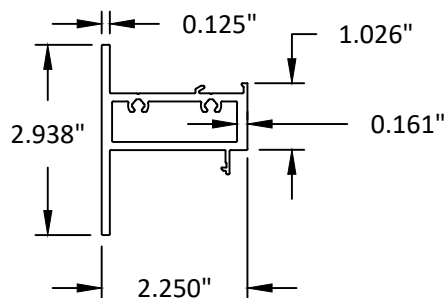
92 MULLION
