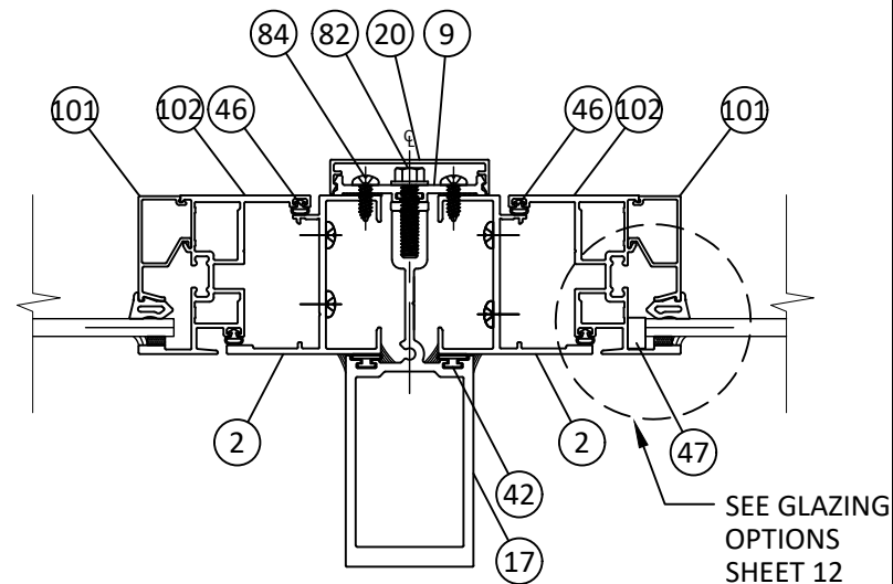
AS 18 HORIZONTAL SECTION STACK MULLION - TYP. "INSWING" CASEMENT TO CASEMENT
