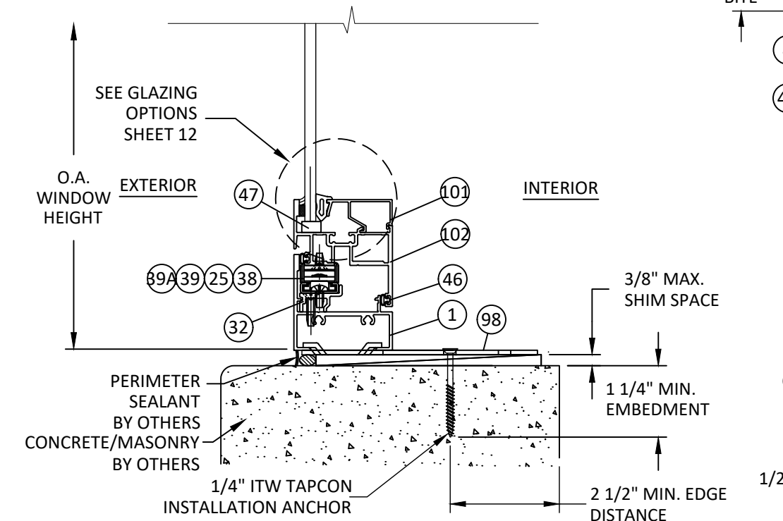
V 12 VERTICAL SECTION VENT SILL - CONCRETE/MASONRY TWIST ANCHOR - TYP. "INSWING"
