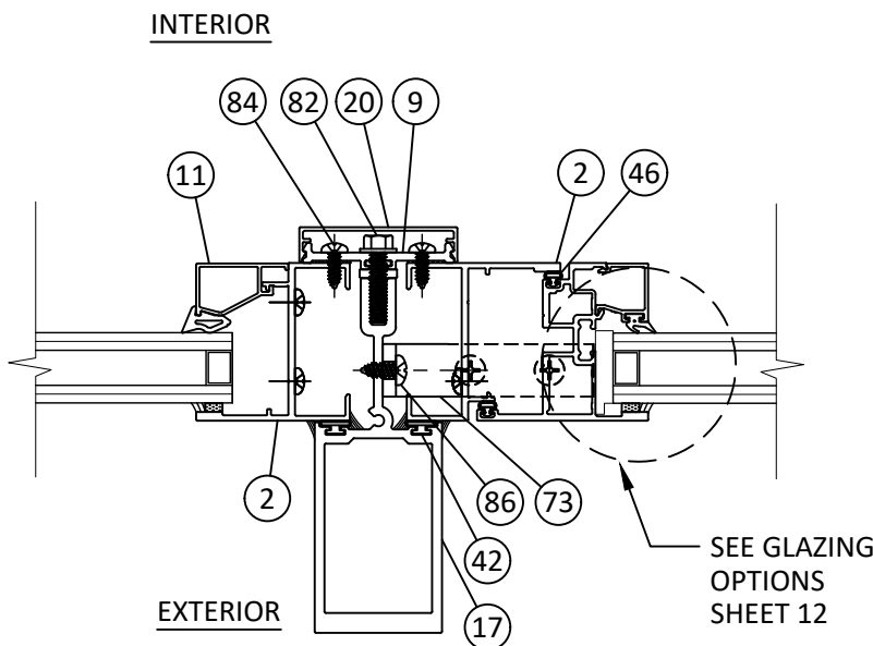
AN HORIZONTAL SECTION 16 STACK MULLION - TYP. FIXED TO CASEMENT "OUTSWING"
