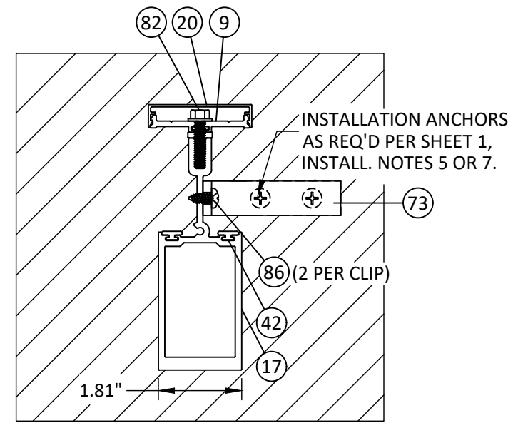
AK HORIZONTAL SECTION 16 STACK MULLION - TYP. JAMB INSTALLATION INSTALL TO WOOD/METAL FRAME
